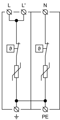
Internal diagram
